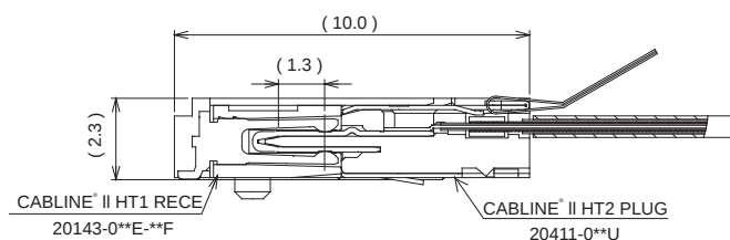
MATED VIEW
